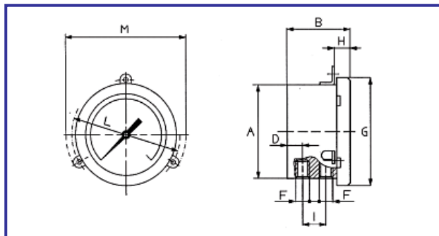
DP gauge for back panel flush mounting with pegs (120° apart)
