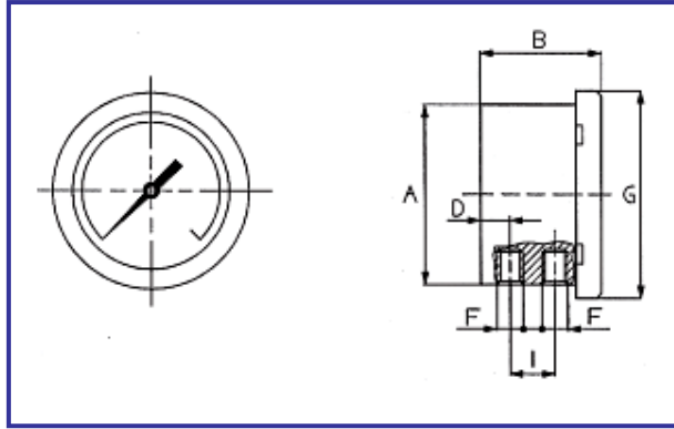
DP gauge for direct mounting
